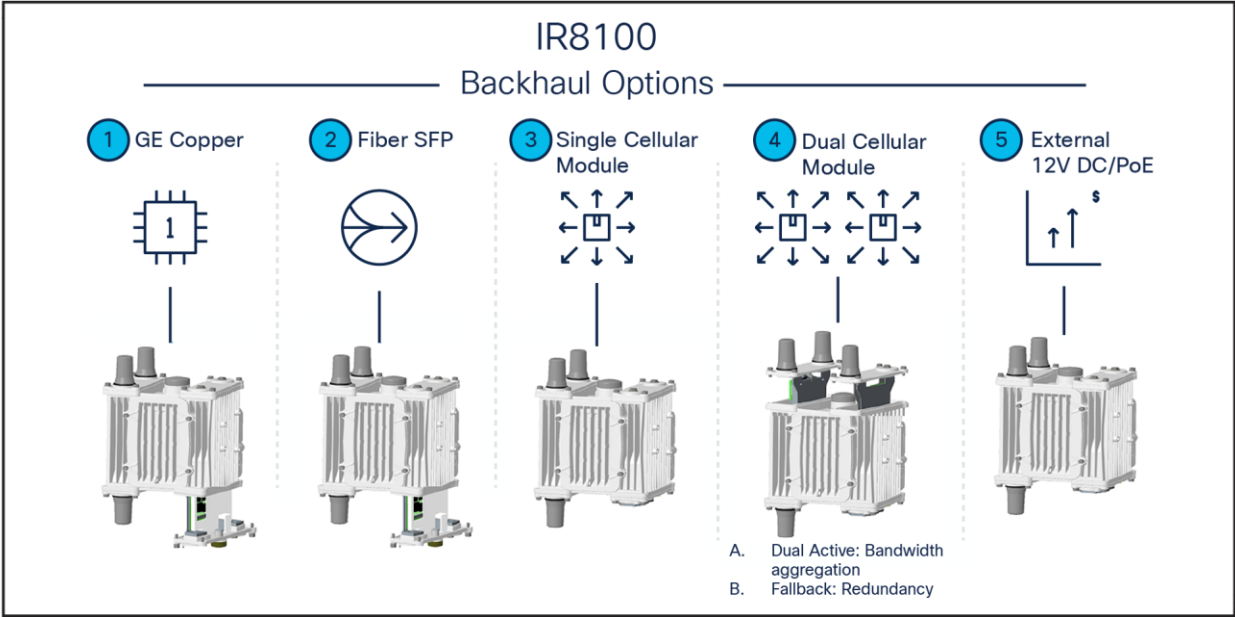
Figure 6. Backhaul options
