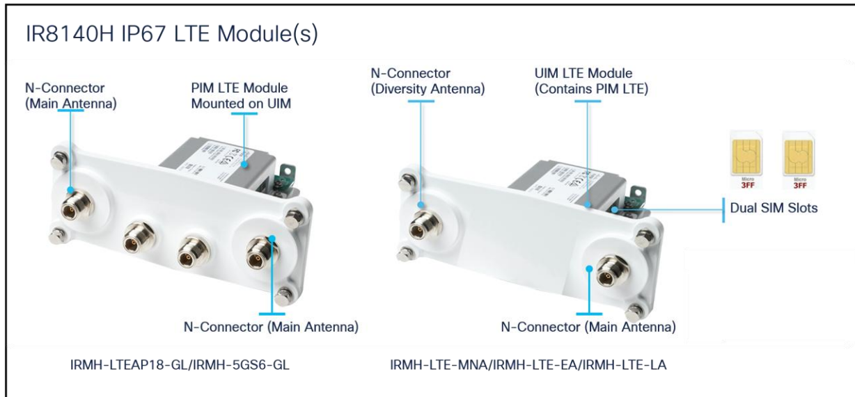
Figure 8. Cellular modules CAT 18, 5G on the left and CAT 4,6 on the right
