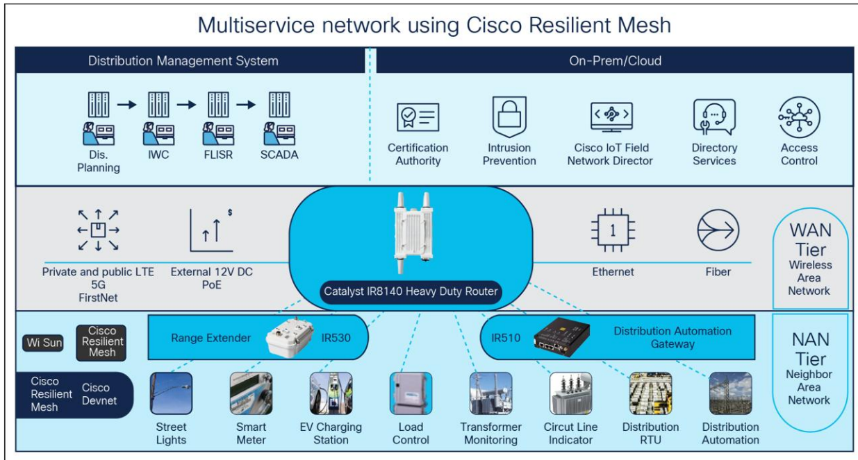
Figure 10. Multiservice network using Cisco Resilient Mesh
