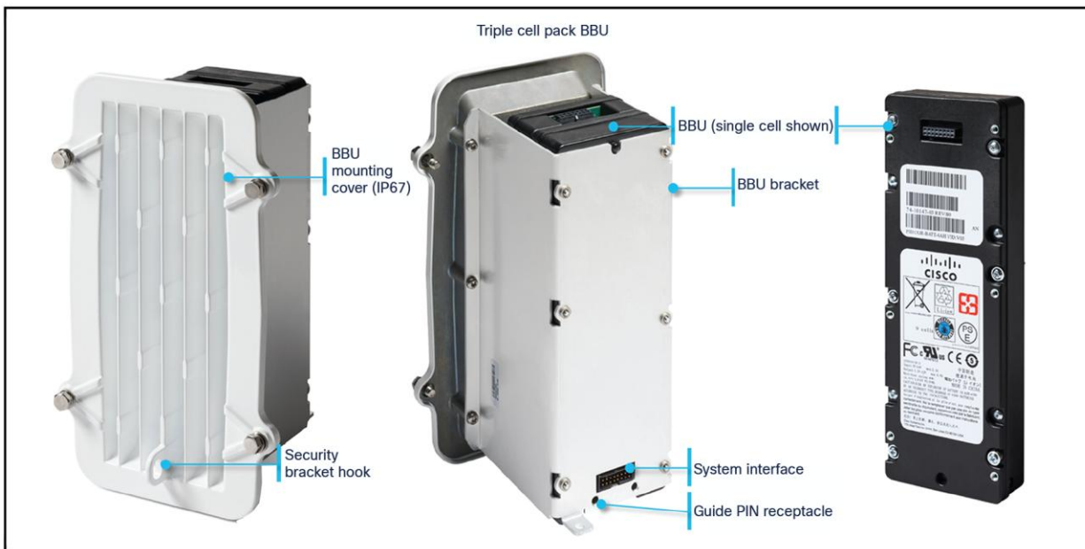
Figure 5. Battery Backup Unit (BBU) module
