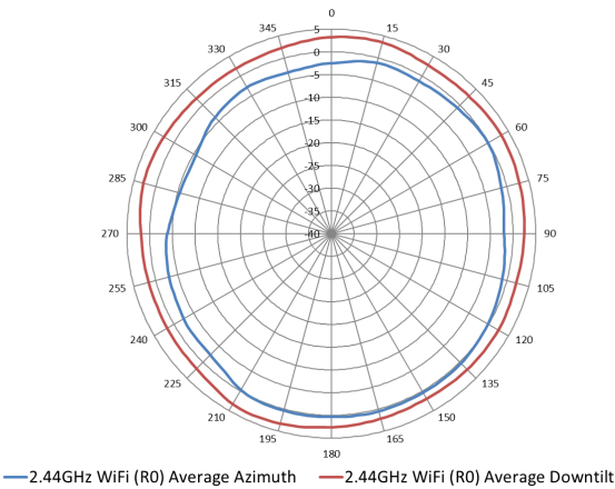
2.44 GHz Wi-Fi antenna patterns (horizontal)
