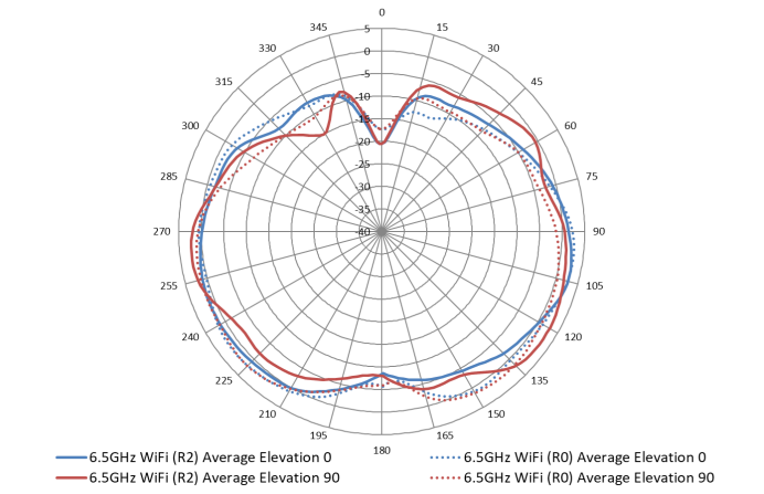
6.5 GHz Wi-Fi antennas patterns (vertical)
