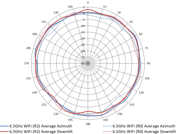
6.5 GHz Wi-Fi antenna patterns (horizontal)
