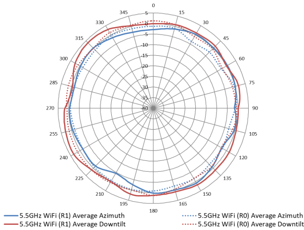
5.5 GHz Wi-Fi antenna patterns (horizontal)
