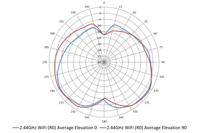
2.44 GHz Wi-Fi antennas patterns (vertical)
