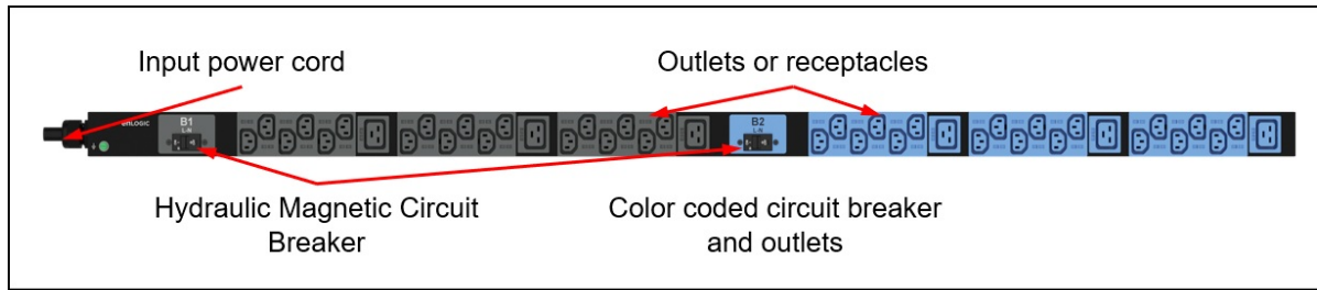
Figure 4. Connectors for Basic PDU (part number 4PU7A93169 or 4PU7A93176)
