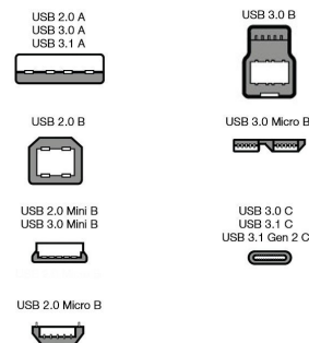
USB Connection Type Reference Chart
