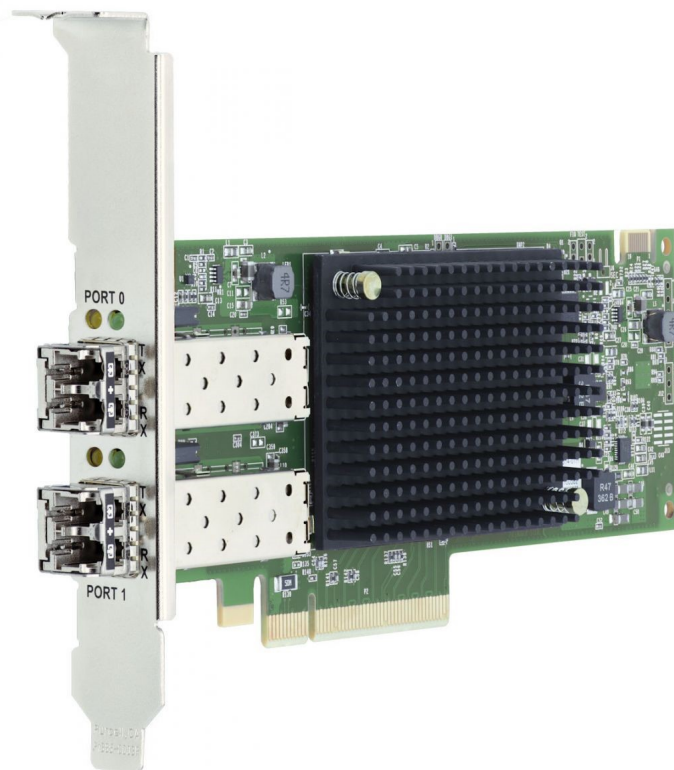
Figure 2. ThinkSystem Emulex LPe37102 32Gb 2-port SecureHBA PCIe Fibre Channel Adapter(Generic FW)
