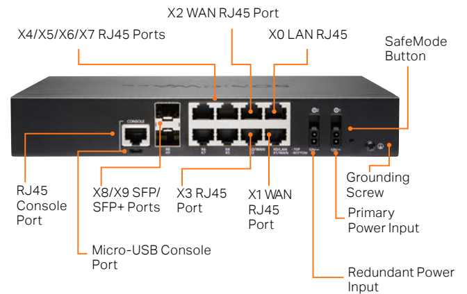
TZ570W Rear Panel
