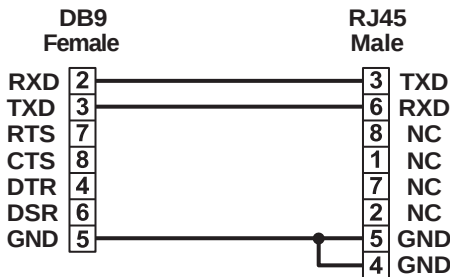
Figure 2.10 Pin Assignment
