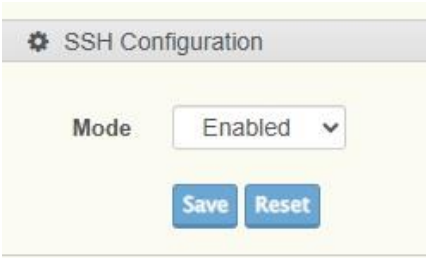
Figure 4.64 SSH Configuration
