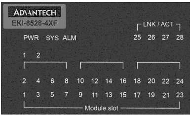
Figure 1.2 System LED Panel
