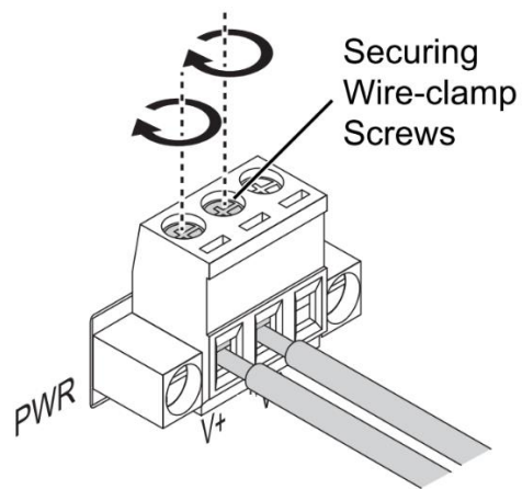
Figure 2.16 Securing DC Wires in a Terminal Block
