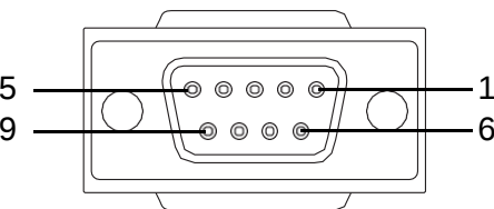
Figure 2.9 DB 9 Pin Position
