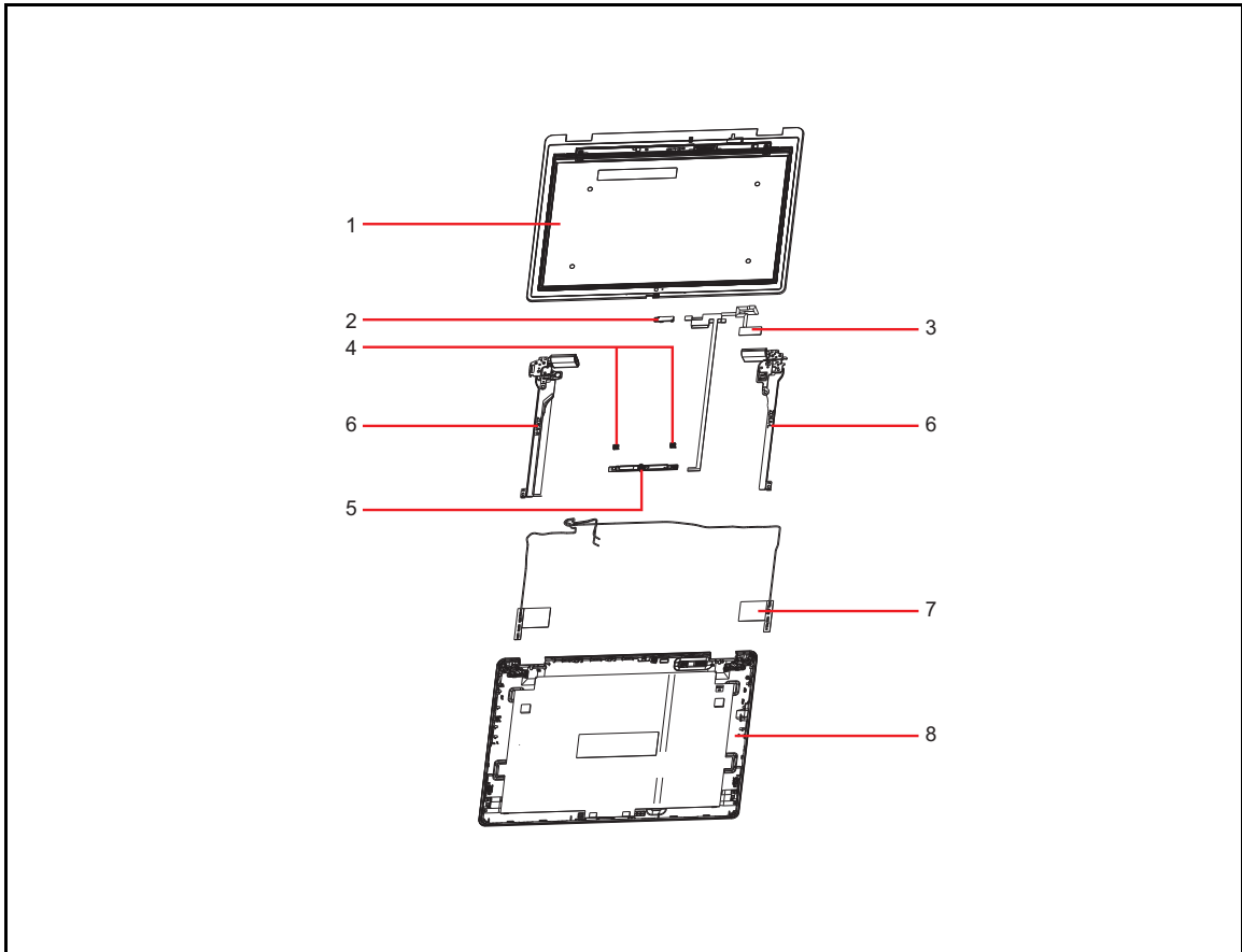
Figure 1-48. LCD Assembly Exploded Diagram
