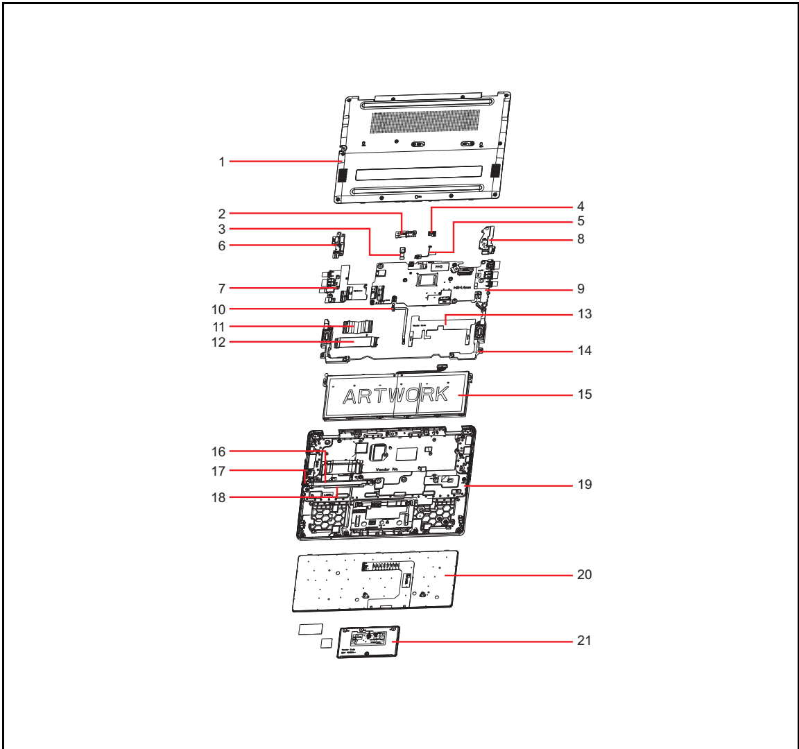
Figure 1-47. System Exploded Diagram
