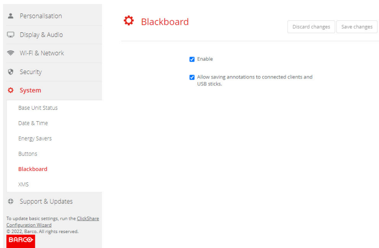
Image 5–54 Save annotations
