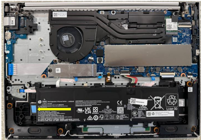
3.22 Slider out from R to L side to release battery
