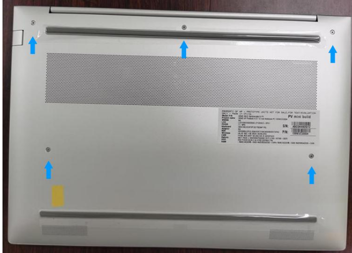
3.21 Use screwdriver to release base cover #1 screw 5PCS
