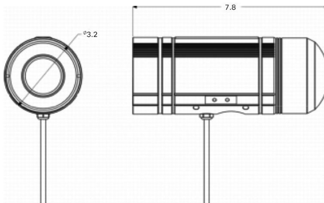
Figure 2. Cisco Video Surveillance 6400 IP Camera Dimensions
