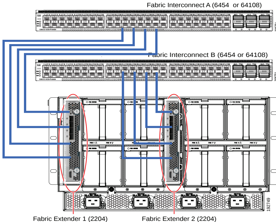
Figure 18 Connecting Blade Chassis Fabric Extenders to Fabric Interconnect Chassis
