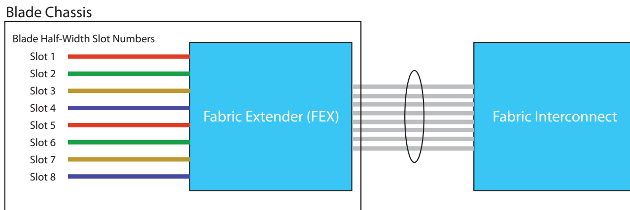
Figure 21 FEX Fabric Links in Port Channel Mode
