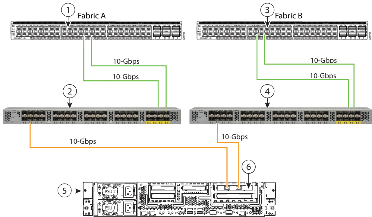
Figure 19 Connecting C-Series Rack Chassis (single-wire management)
