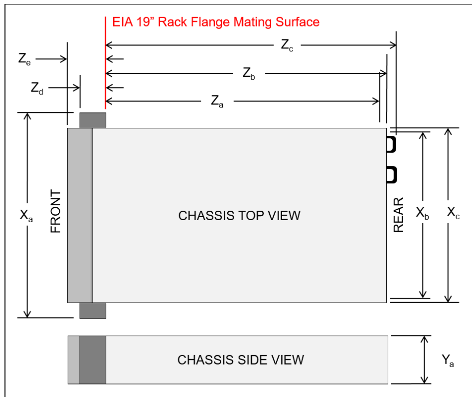
Figure 28. Server dimensions
