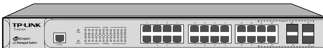
Figure 2-1 Front Panel of TL-SG3424
