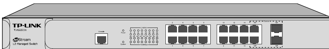
Figure 2-1 Front Panel of TL-SG3216
