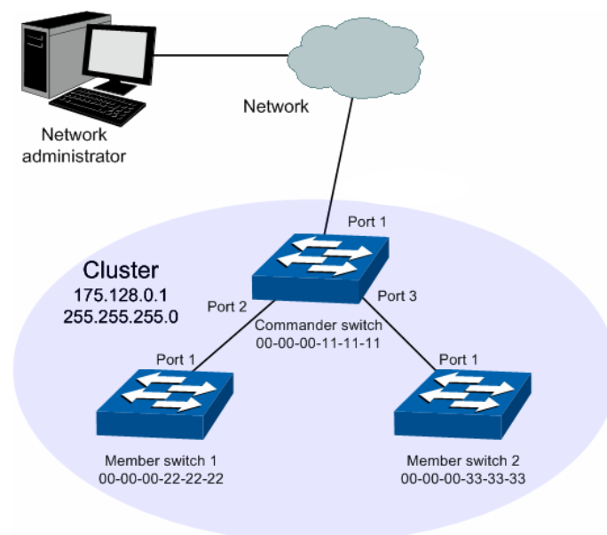
Figure 13-15 Network diagram
