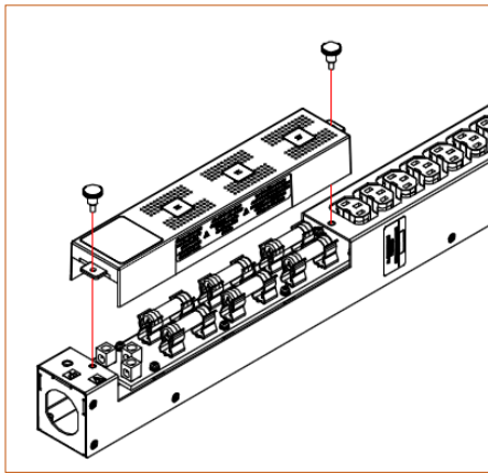
Figure 4-A. Fuse Cover Removal
