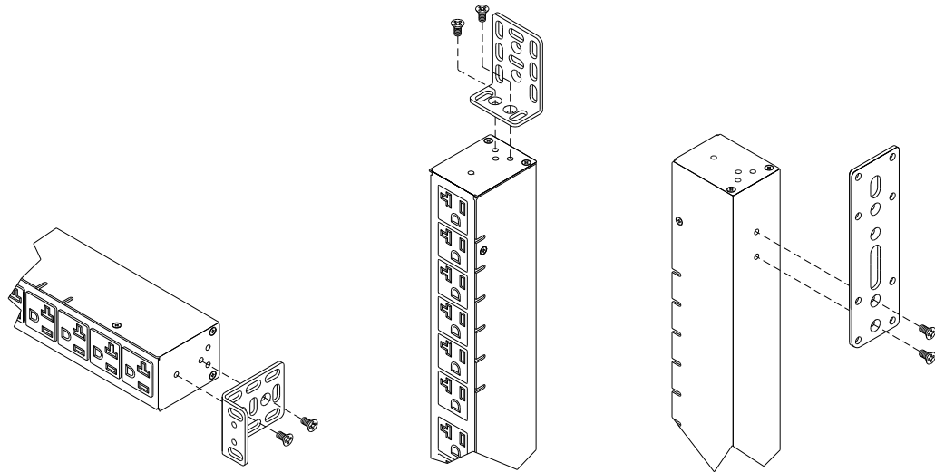
Figure 3. Mounting Views
