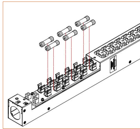
Figure 4-B. Fuse Removal
