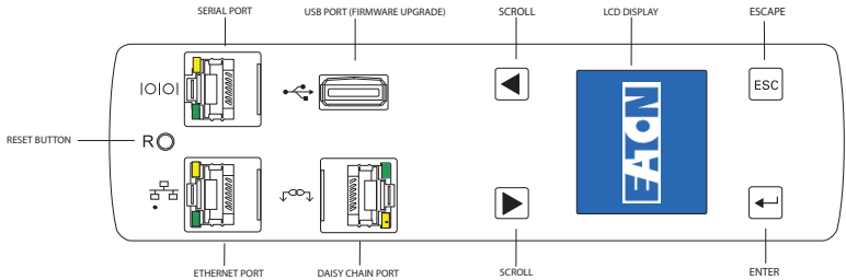
Figure 1. ePDU LCD Front Panel Window and Buttons
