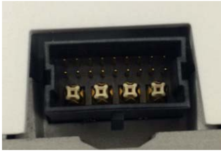
Figure 8 Smart Antenna Connector 3802E Model
