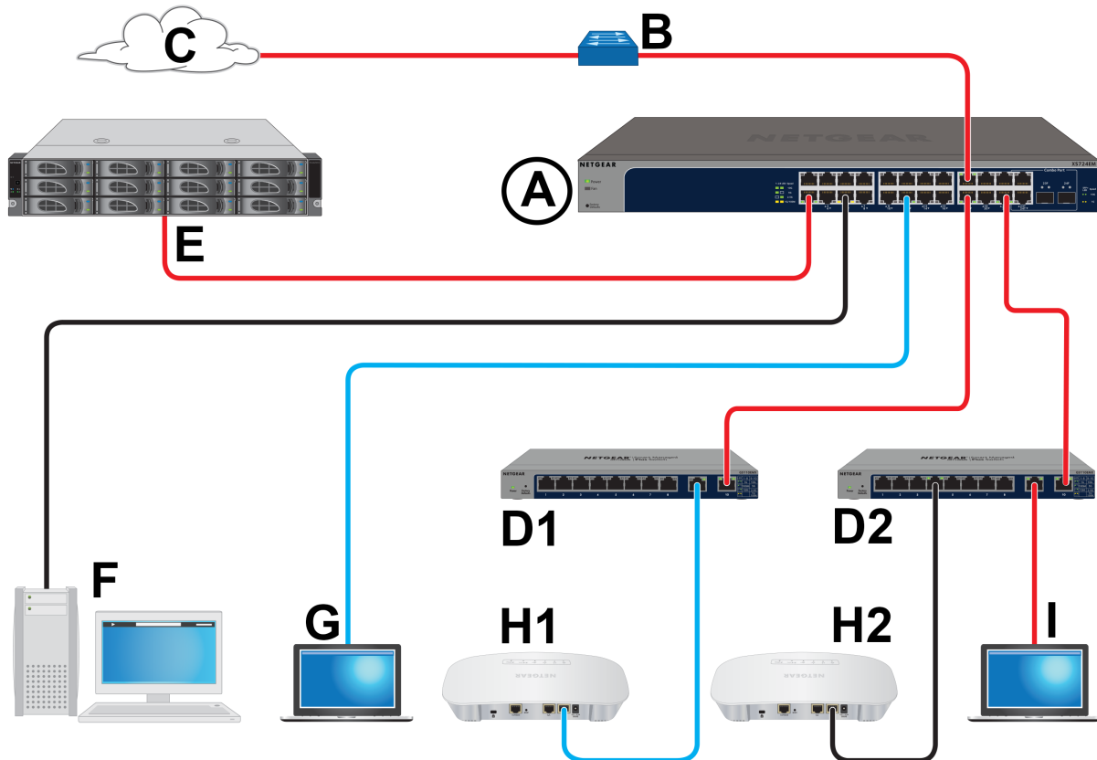
Figure 6. Sample connections
