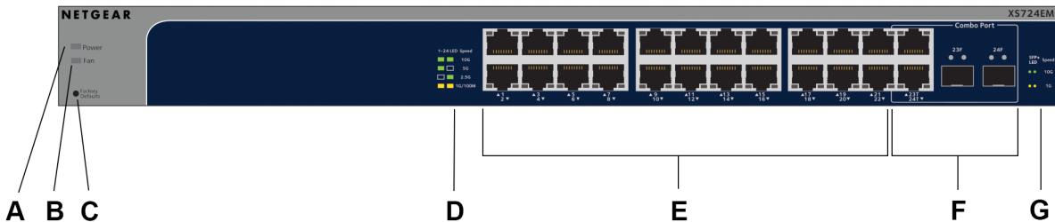
Figure 2. Front panel model XS724EM
