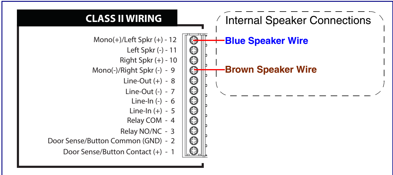
Figure 2-4. SIP IP66 Outdoor Horn Connections
