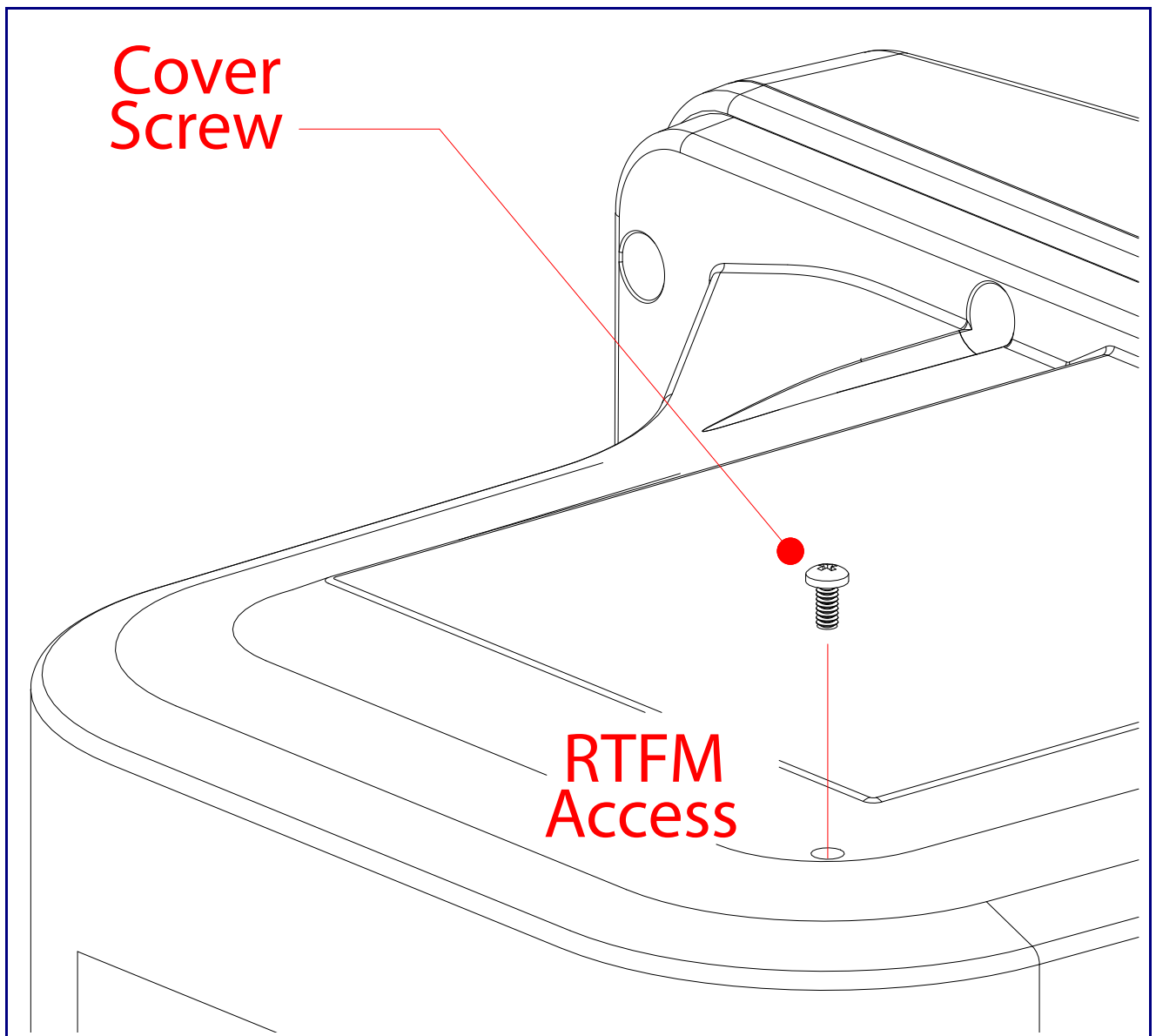
Figure 2-7. RTFM Switch
