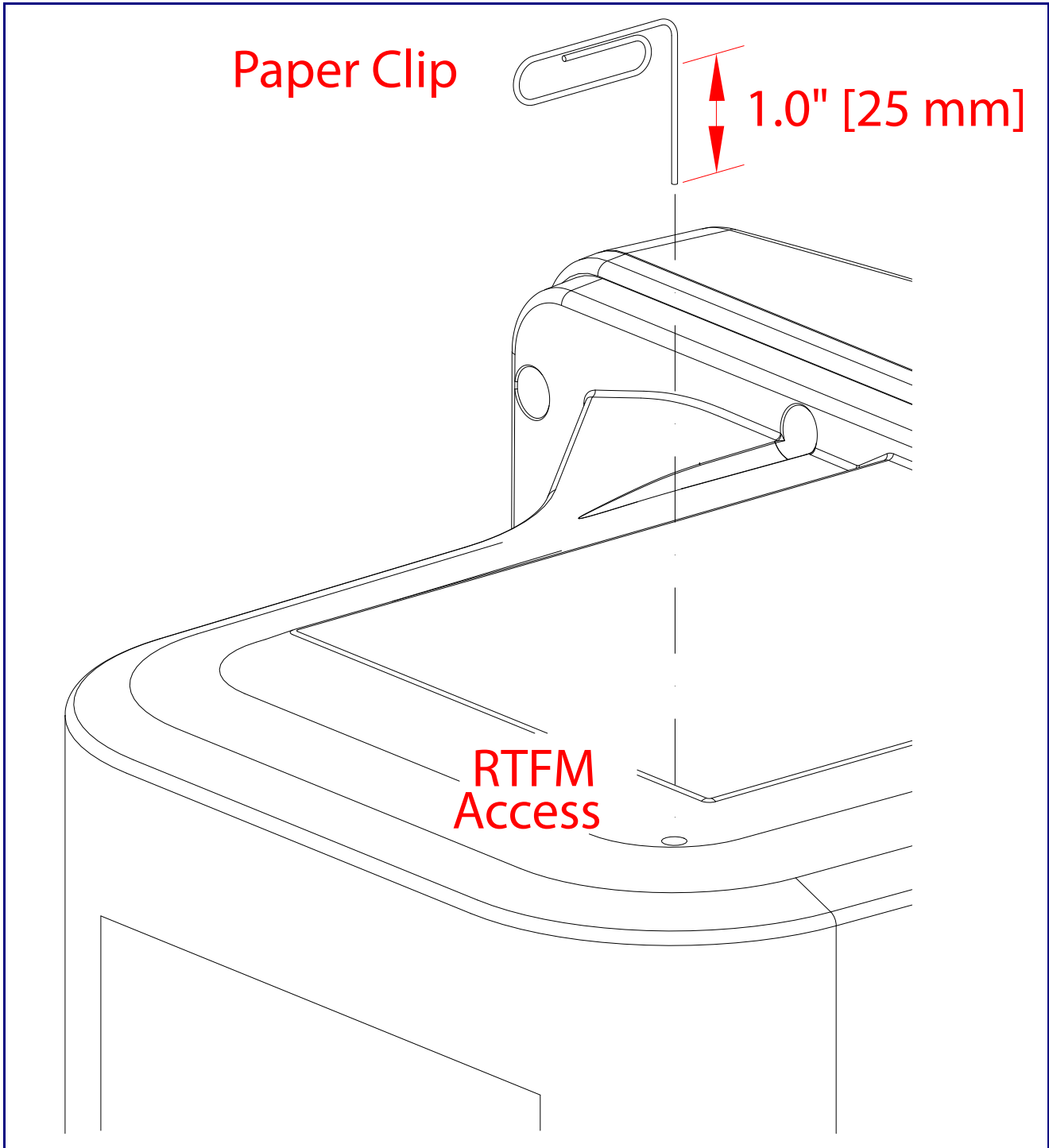
Figure 2-8. RTFM Switch
