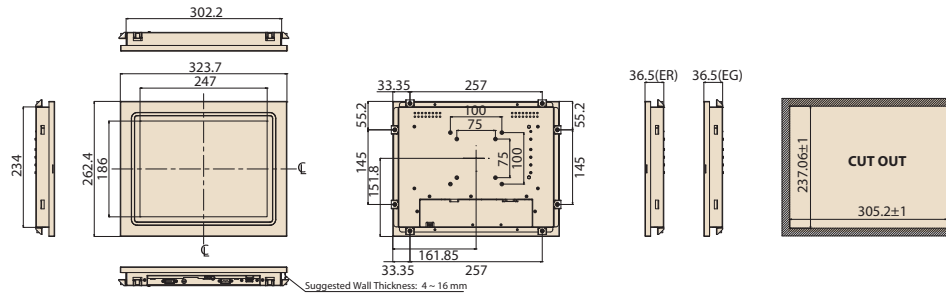
Figure 2.3 IDS-3212E (SVGA) Series Dimensions
