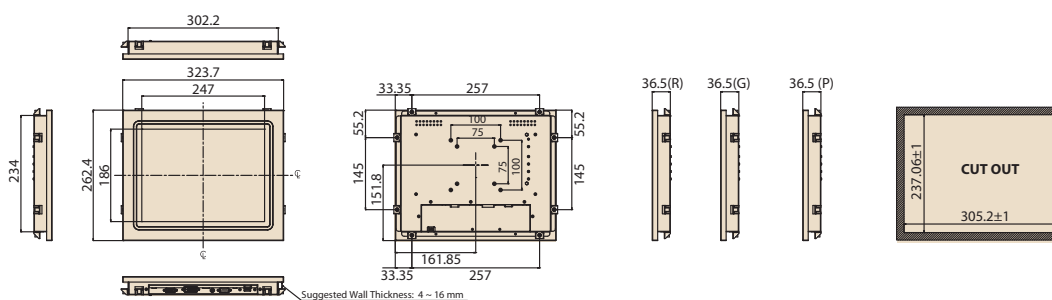
Figure 2.1 IDS-3212 (XGA) Series Dimensions
