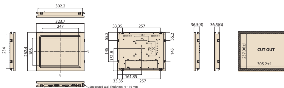
Figure 2.2 IDS-3212 (SVGA) Series Dimensions
