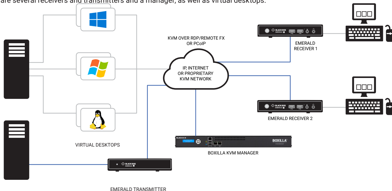
EMERALD SWITCHING EXAMPLE
