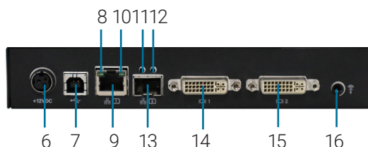
REAR VIEW OF EMD2002PE-T-R2
