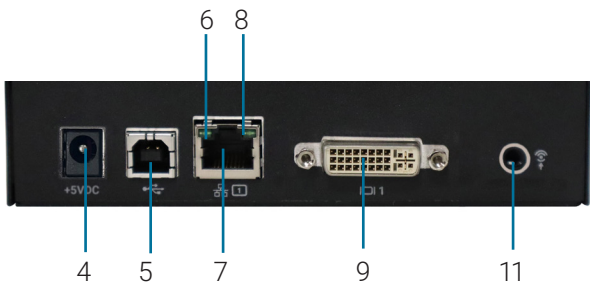
REAR VIEW OF THE EMERALD SE R2 DVI TRANSMITTER, DUAL-HEAD (EMD2000SE-T-R2)
