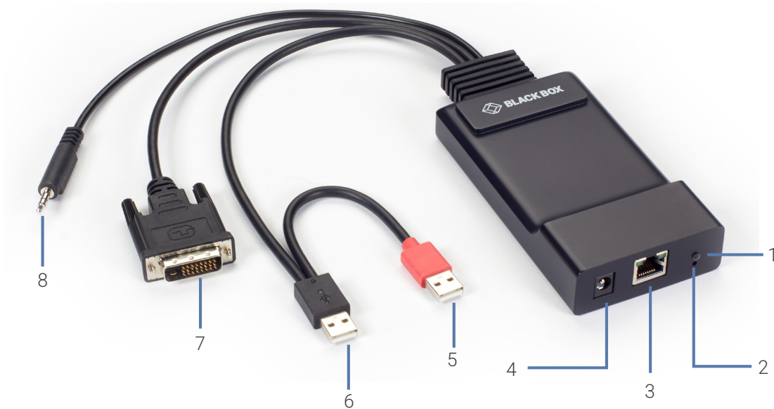
FRONT VIEW OF THE EMERALD ZEROU DVI TRANSMITTER, SINGLE-HEAD (EMD200DV-T)
