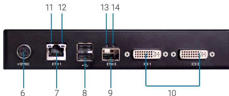
REAR VIEW OF EMERALD PE RECEIVER, DUAL-HEAD (EMD2002PE-R, EMD2002PE-R-P)
