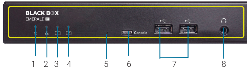
FRONT VIEW OF THE EMERALD PE RECEIVER, DUAL-HEAD (EMD2002PE-DP-R)
