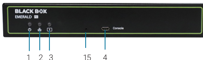
FRONT VIEW OF EMD2000PE-T-R2
