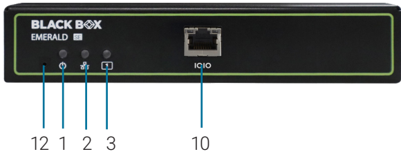
FRONT VIEW OF THE EMERALD SE R2 DVI TRANSMITTER, DUAL-HEAD (EMD2000SE-T-R2)
