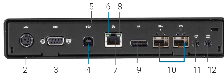
REAR VIEW OF THE EMERALD 4K TRANSMITTER (EMD4000T)
