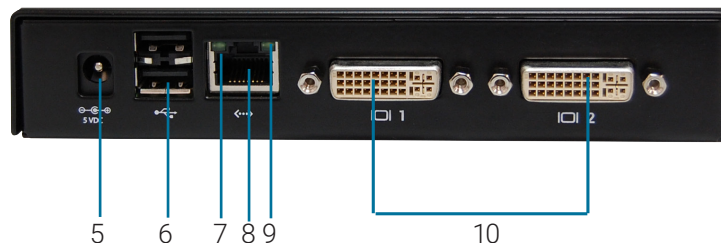
REAR VIEW OF EMERALD SE RECEIVER, DUAL-HEAD (EMD2002SE-R)
