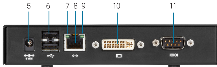
REAR VIEW OF EMERALD SE RECEIVER, SINGLE-HEAD (EMD2000SE-R)
