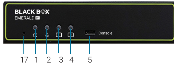
FRONT VIEW OF THE EMERALD PE TRANSMITTER, DUAL-HEAD (EMD2002PE-DP-T)
