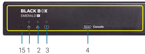
FRONT VIEW OF THE EMERALD PE TRANSMITTER, SINGLE-HEAD (EMD2000PE-DP-T)
