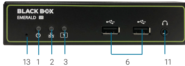
FRONT VIEW OF EMERALD SE DP RECEIVER, SINGLE-HEAD (EMD2000SE-DP-R)
