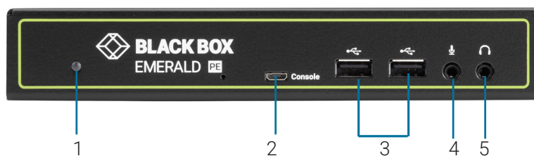
FRONT VIEW OF EMERALD PE RECEIVER, SINGLE-HEAD (EMD2000PE-R, EMD2000PE-R-P)
