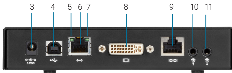
REAR VIEW OF THE EMERALD SE TRANSMITTER, SINGLE-HEAD (EMD2000SE-T (EOL))
