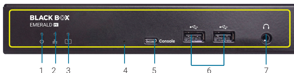
FRONT VIEW OF THE EMERALD PE RECEIVER, SINGLE-HEAD (EMD2000PE-DP-R)
