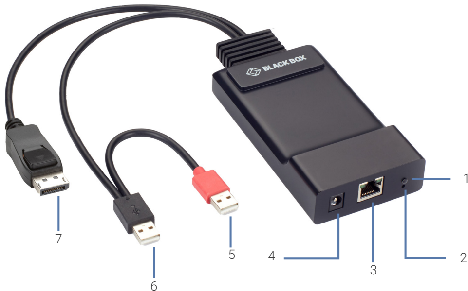
FRONT VIEW OF THE EMERALD ZERO DP TRANSMITTER, SINGLE-HEAD (EMD200DP-T)
