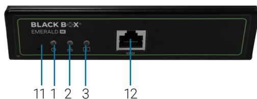
FRONT VIEW OF THE EMERALD SE TRANSMITTER, SINGLE-HEAD (EMD2000SE-DP-T)
