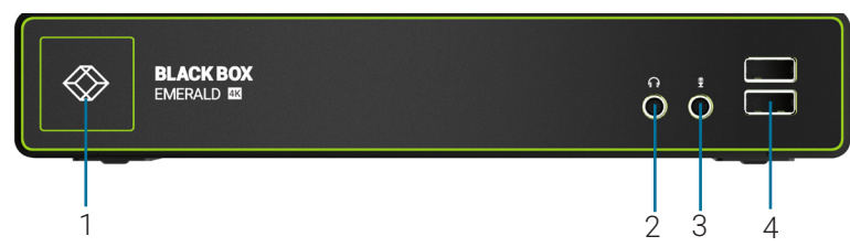
FRONT VIEW OF EMERALD 4K RECEIVER (EMD4000R)
