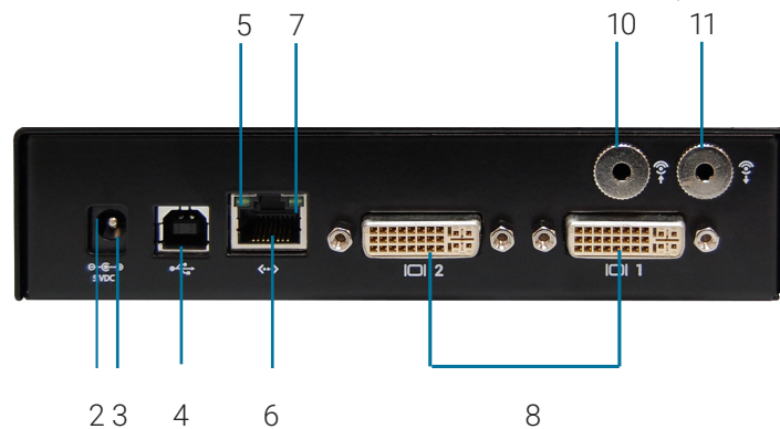
REAR VIEW OF THE EMERALD SE TRANSMITTER, DUAL-HEAD (EMD2002SE-T (EOL))
