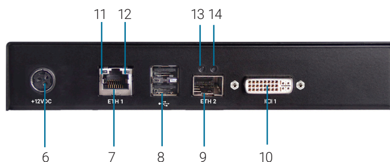
REAR VIEW OF EMERALD PE RECEIVER, SINGLE-HEAD (EMD2000PE-R, EMD2000PE-R-P)
