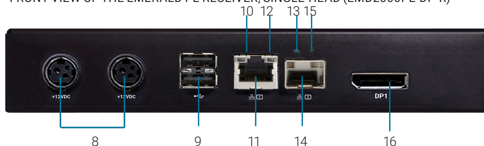
FRONT VIEW OF THE EMERALD PE RECEIVER, SINGLE-HEAD (EMD2000PE-DP-R)
