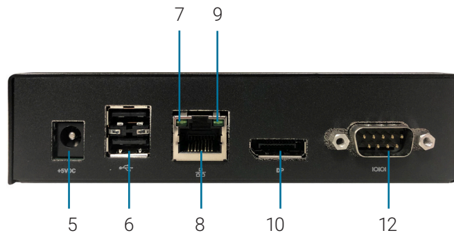
REAR VIEW OF EMERALD SE DP RECEIVER, SINGLE-HEAD (EMD2000SE-DP-R)
