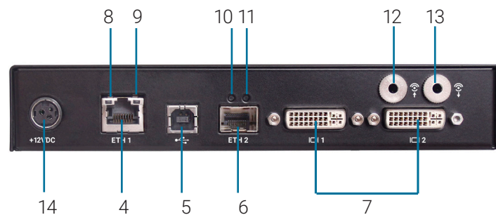
REAR VIEW OF THE EMERALD PE TRANSMITTER, DUAL-HEAD (EMD2002PE-T (EOL), EMD2002PE-T-P (EOL))
