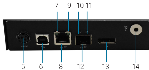
REAR VIEW OF THE EMERALD PE TRANSMITTER, SINGLE-HEAD (EMD2000PE-DP-T)
