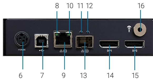
FRONT VIEW OF THE EMERALD PE TRANSMITTER, DUAL-HEAD (EMD2002PE-DP-T)
