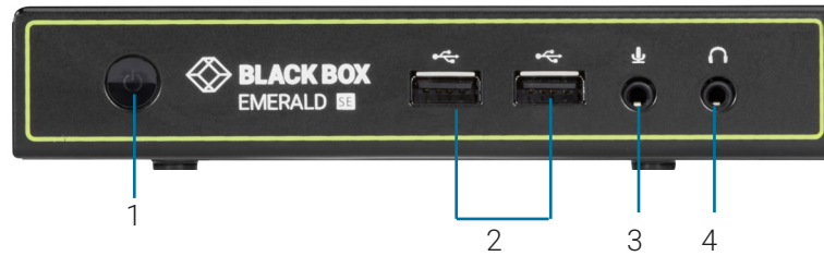
FRONT VIEW OF EMERALD SE RECEIVER, SINGLE-HEAD (EMD2000SE-R)
