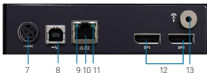
REAR VIEW OF THE EMERALD SE TRANSMITTER, DUAL-HEAD (EMD2002SE-DP-T)
