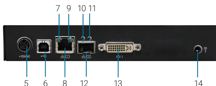
REAR VIEW OF EMD2000PE-T-R2
