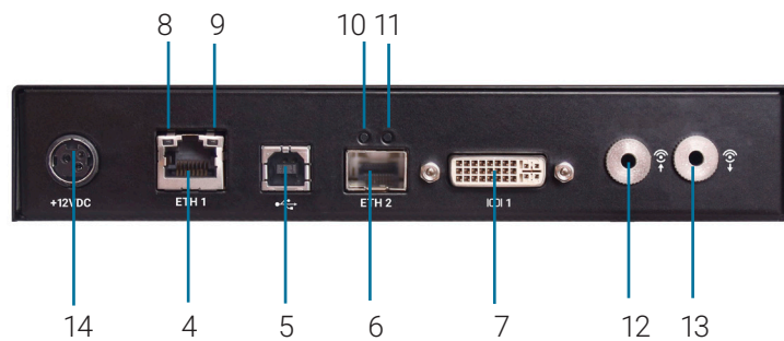
REAR VIEW OF THE EMERALD PE TRANSMITTER, SINGLE-HEAD (EMD2000PE-T (EOL), EMD2000PE-T-P (EOL))
