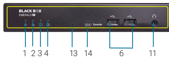
FRONT VIEW OF EMERALD SE DP RECEIVER, DUAL-HEAD (EMD2002SE-DP-R)
