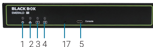
FRONT VIEW OF EMD2002PE-T-R2
