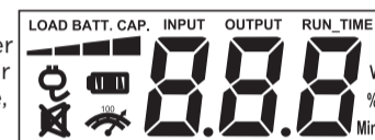
The LCD display indicates a variety of UPS operational conditions. All descriptions apply when the UPS is plugged into an AC outlet and turned on or when the UPS is on battery.
