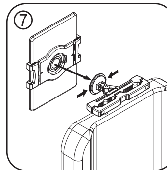
Press side buttons, attach bracket, release buttons, and spin until you hear the click.
