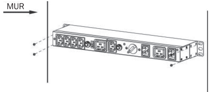
Figure 2 : montage mural
