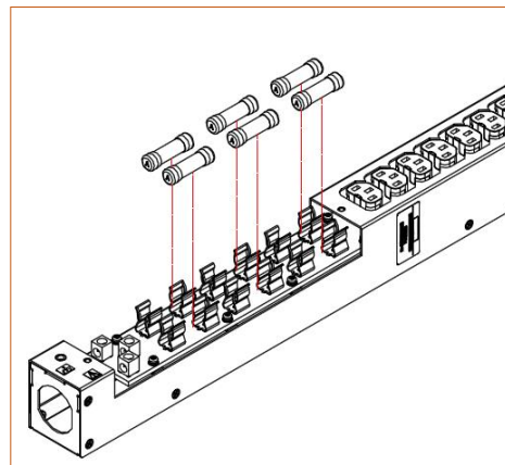
Figure 2. Fuse Removal
