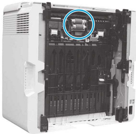
Figure 9-17 Clean the rollers
