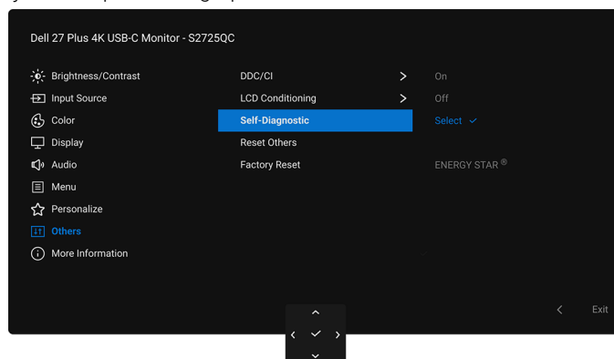
Figure 76. Self-Diagnostic menu
