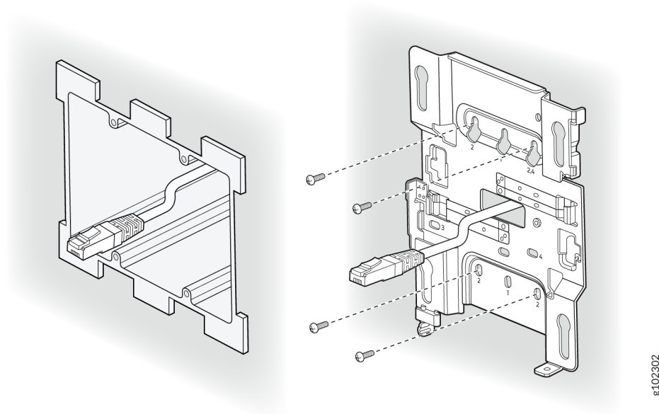
Figure 8: Attach the APBR-U Mounting Bracket to the Double-Gang Junction Box
